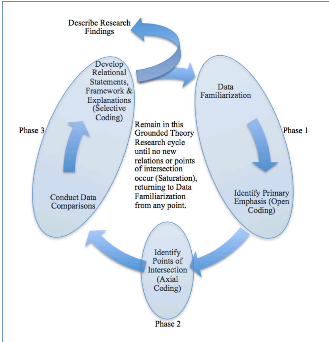
Figure 10. Research Method
